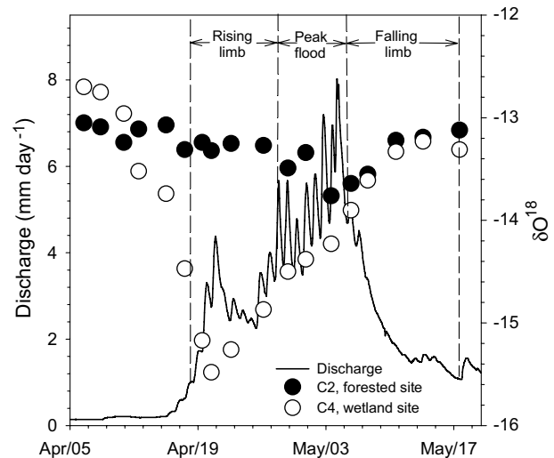
Figure 2 Spring flood discharge at catchment, C7, defining the rising limb, peak flood and falling limb periods as used in this study. Oxygen-18 ( \delta^{18}\text{O} ) values for catchments C2 and C4 are shown.
