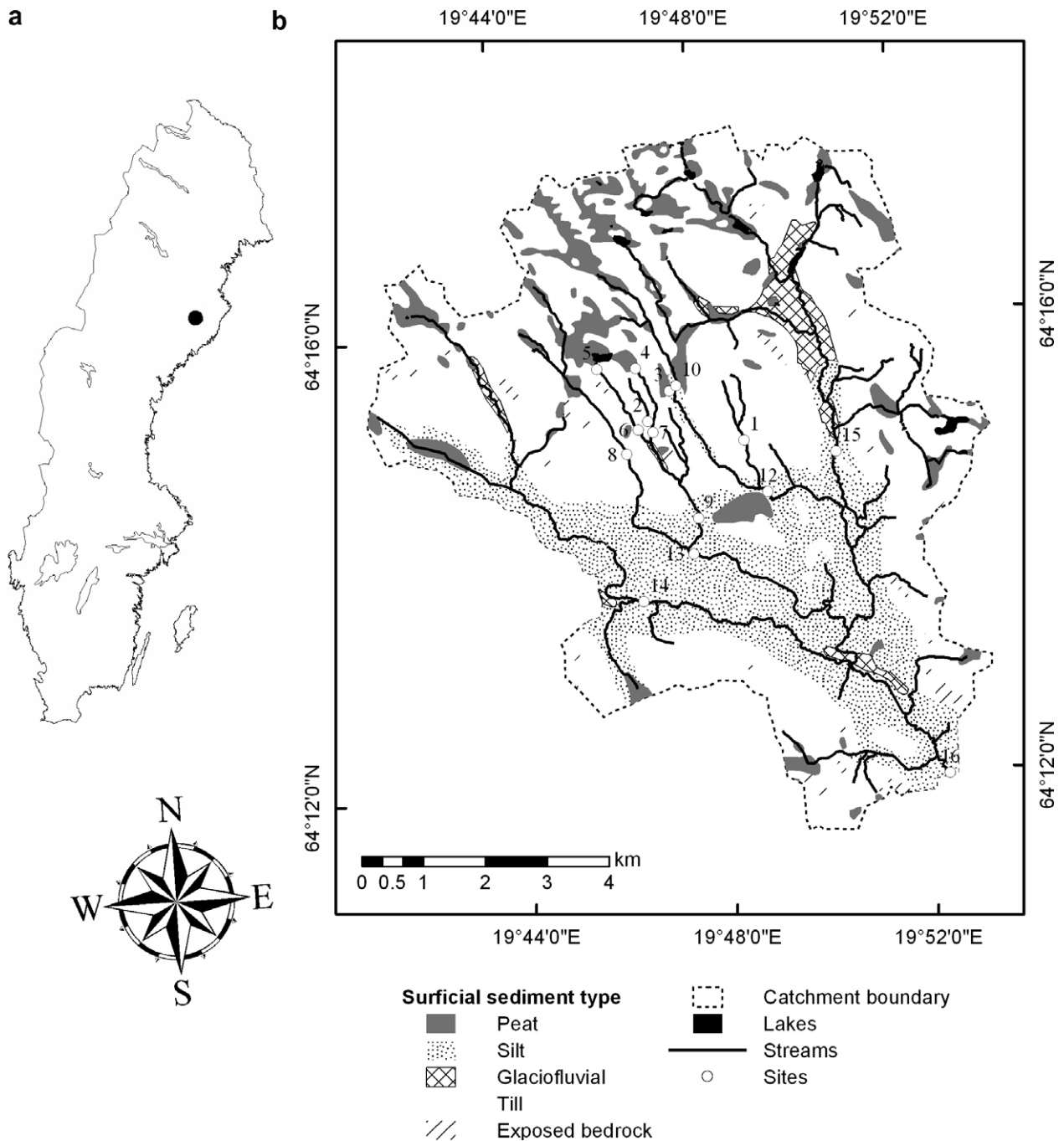
Figure 1 Location of the Krycklan catchment in northern Sweden (a), and distribution of major surficial sediment types and location of stream study sites within the catchment (b).
