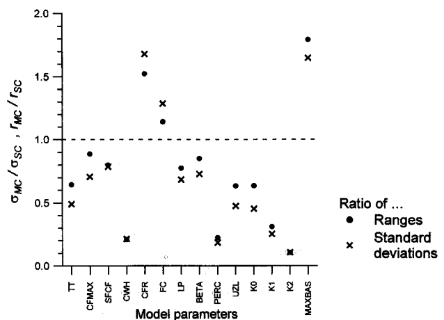
Fig. 3. Comparison of the variations of calibrated parameter values obtained by single- and multi-criteria calibration of the HBV model in the Lilla Tivsjön catchment. Both ranges and standard deviations were calculated from the 20 best of 25 calibration trials. The ratios were computed by dividing those values for standard deviation and range from calibrations against both runoff and groundwater levels, \sigma_{MC} and r_{MC} , by the values from calibration against only runoff, \sigma_{SC} and r_{SC} .
