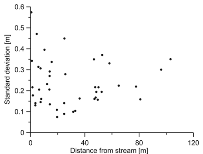
Figure 8. Standard deviation of the relative differences between local groundwater levels and the hillslope average level (for different points in time) versus distance of the well from the stream.
