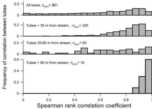
Figure 6. Frequency distribution for the rank correlation coefficients for all pairs of wells and all pairs of wells that are located less than 35 m, between 35 and 60 m, and more than 60 m from the stream.
