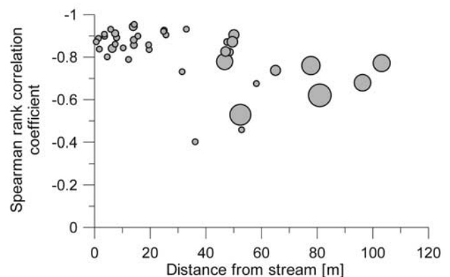
Figure 5. Strongest rank correlation between groundwater levels and runoff versus distance from the stream when shifting the groundwater-level time series in time. The area of the bubbles is proportional to the time shift needed to obtain the strongest correlation varying from 0 (smallest bubbles) to 80 hours.
