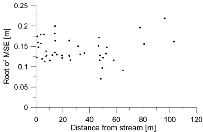
Figure 7. Root of mean squared error of the model z_{i,t} = a_0 + b_i + c_t + \varepsilon against distance from the stream for each well.
